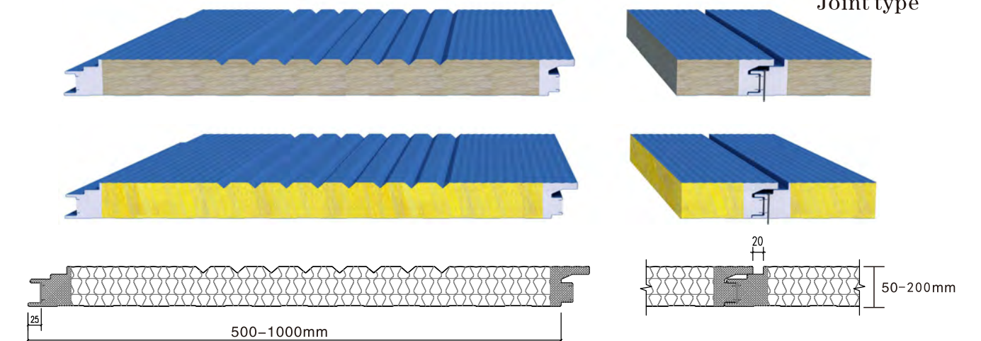
Joint type
