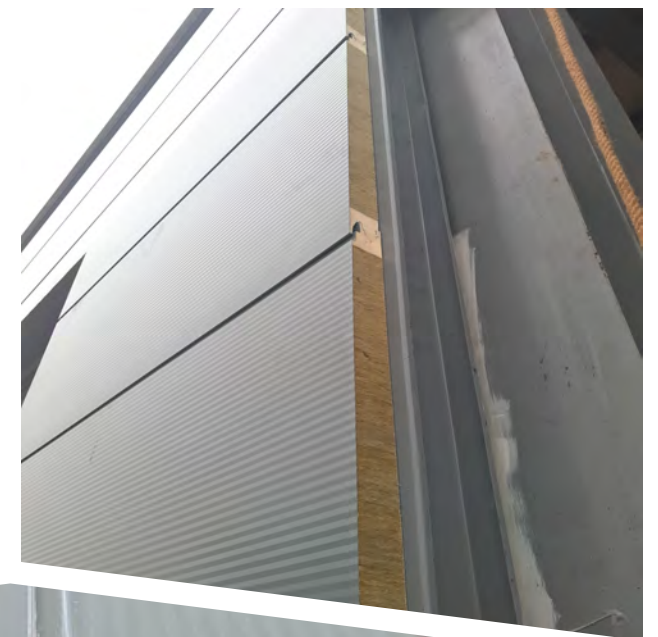
Joint without gap for horizontal application
