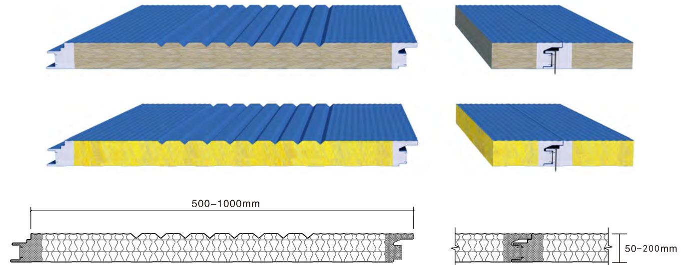
Joint type
